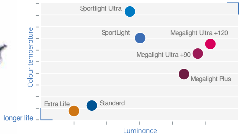
Colour temperature-luminance-life comparisons for the premium range
